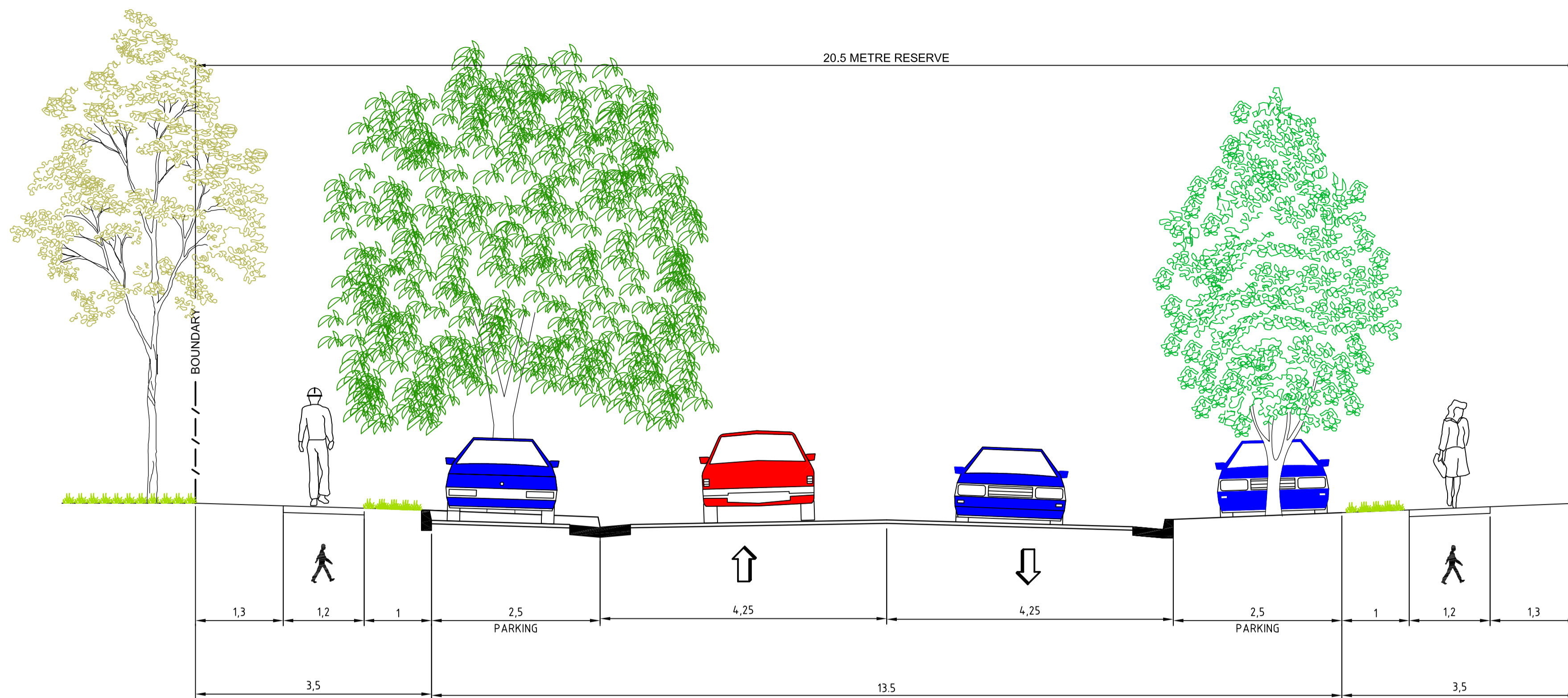
20.5m ROAD RESERVE (INDUSTRIAL OTHER)
